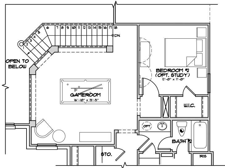
ALT. GAMEROOM/BEDROOM LAYOUT
