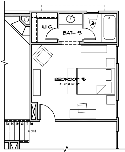
OPT. BED/BATH LAYOUT #2
