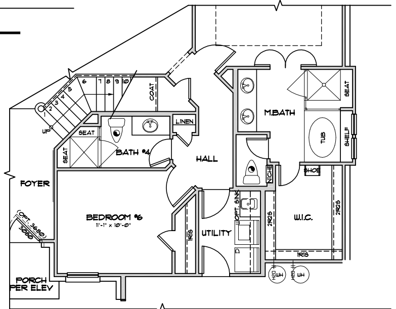
OPT. BED/BATH LAYOUT #3
